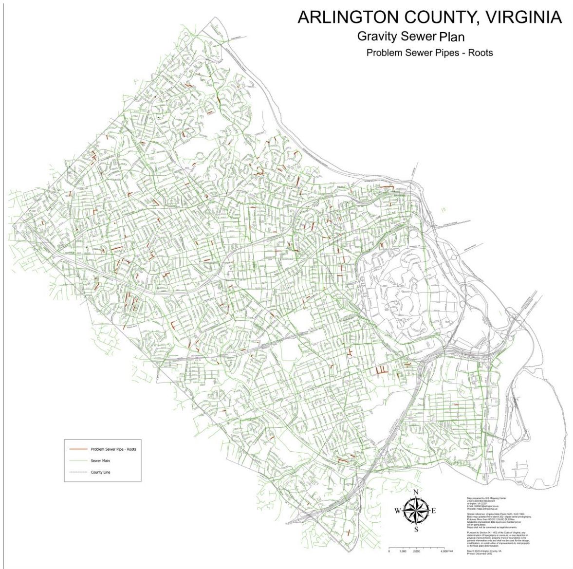
Figure 2-7 Sewer Segments Regularly Treated to Control Roots
