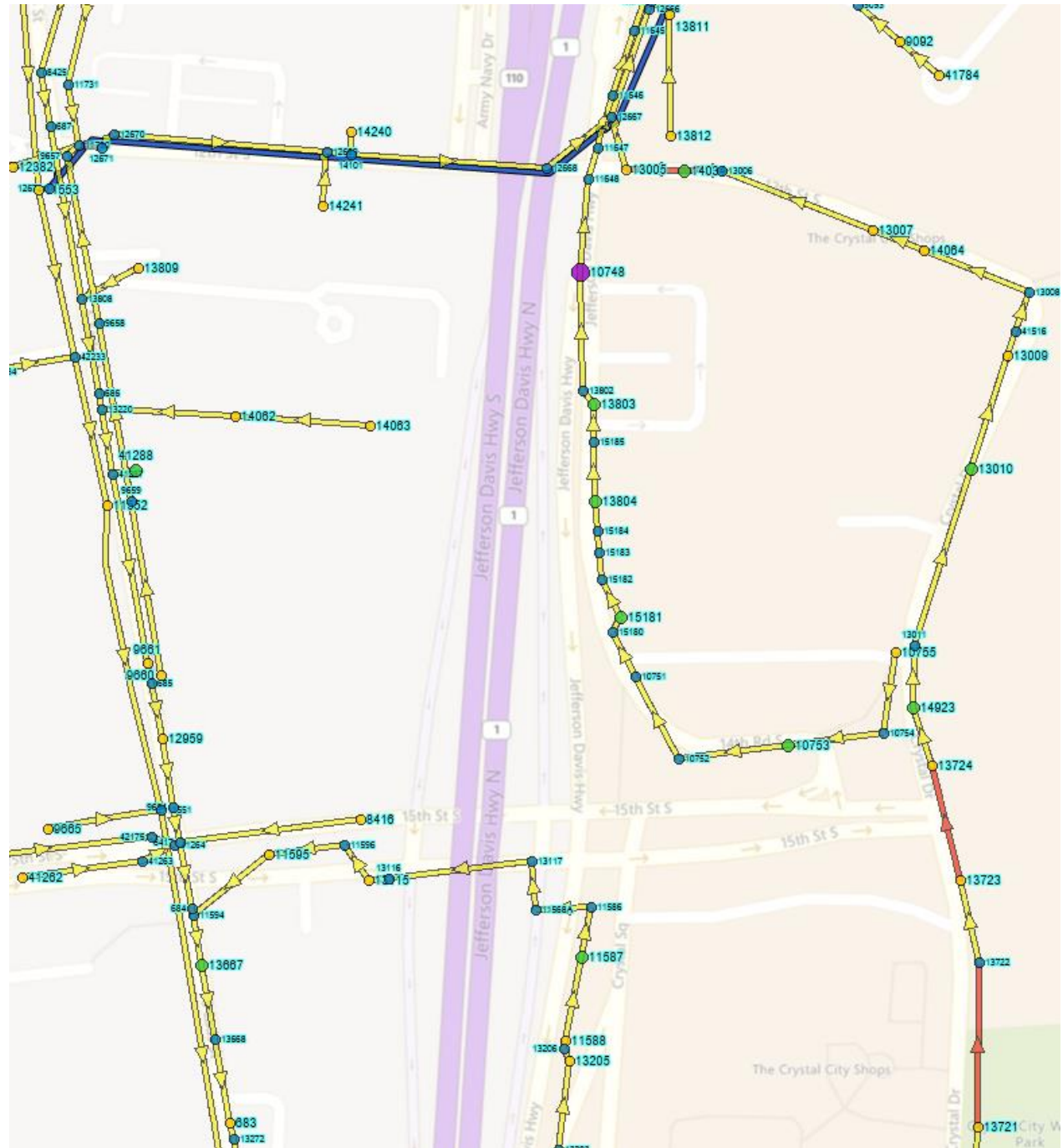
Figure 3-10. >90% Full-Flow Sewer Segments Along Crystal Drive in National Landing, Future 4X Planning Scenario
