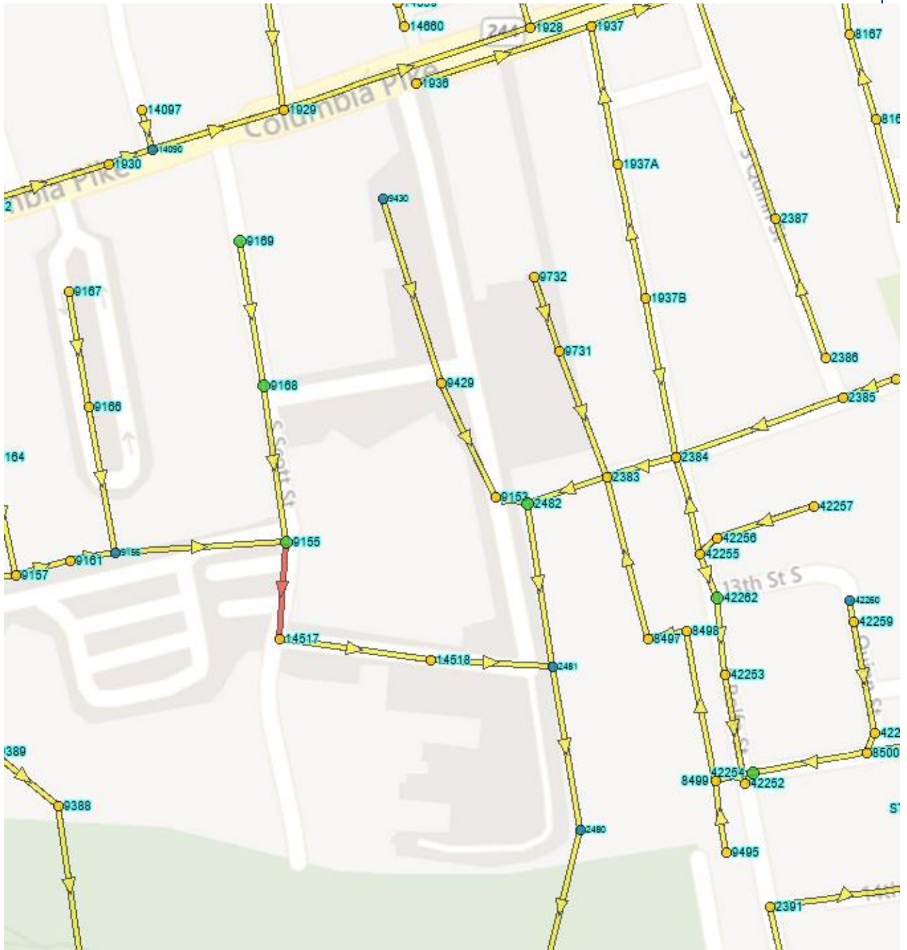
Figure 3-15. >90% Full-Flow Sewer Segment Along S. Scott St in Columbia Heights, Future 4X Planning Scenario
